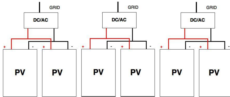
Figure 4. Schematic of system 3 (Micro inverters)
