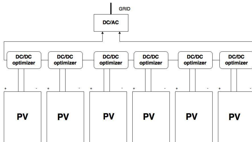
Figure 3. Schematics of System 2 (String inverter with additional DC/DC optimizers)
